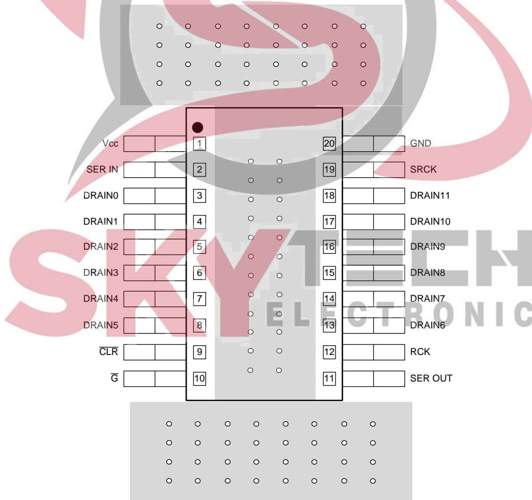
Figure 15. Layout Recommendation
